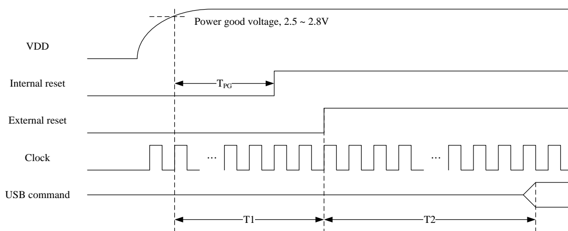
Figure 5.4 - Power on Sequence of GL850G
